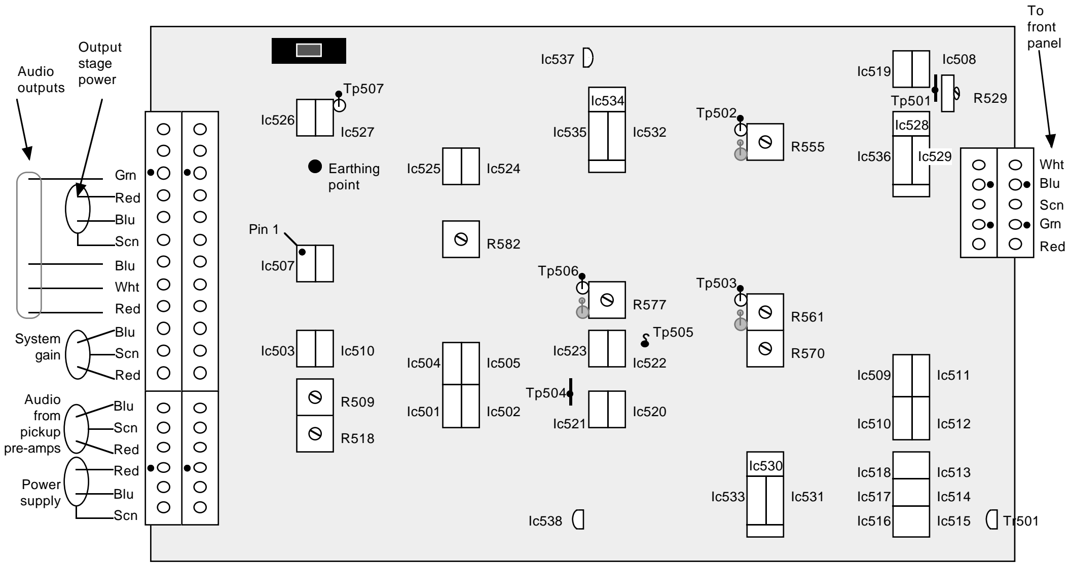
AUDIO BOARD
